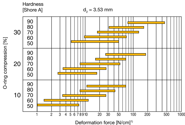
1) Length of O-ring circumference (cm) Fig. 8.28
