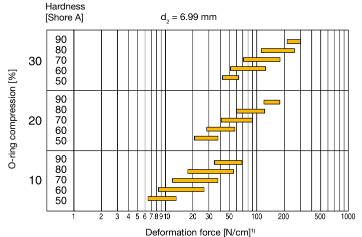
1) Length of O-ring circumference (cm) Fig. 8.30
