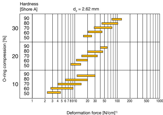
1) Length of O-ring circumference (cm) Fig. 8.27
