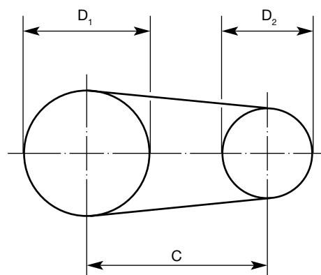
Fig. 2.19 Open design
