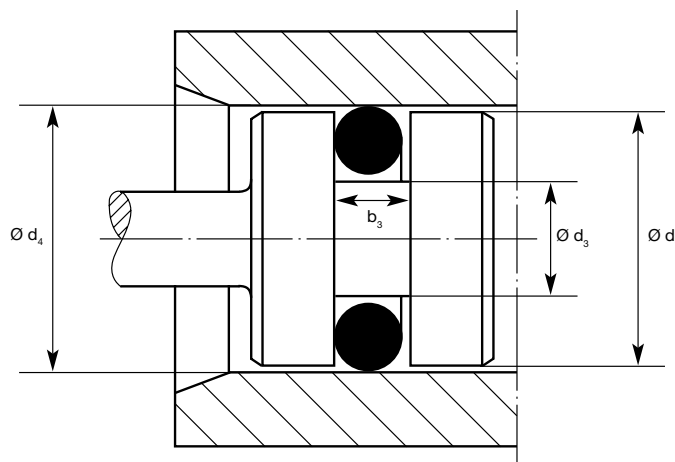
Fig. 3.15 Floating design – no compression
