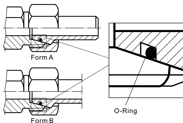
Fig. 4.4 Assembly
