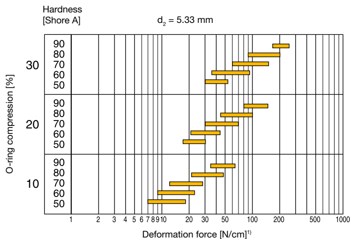
1) Length of O-ring circumference (cm) Fig. 8.29
