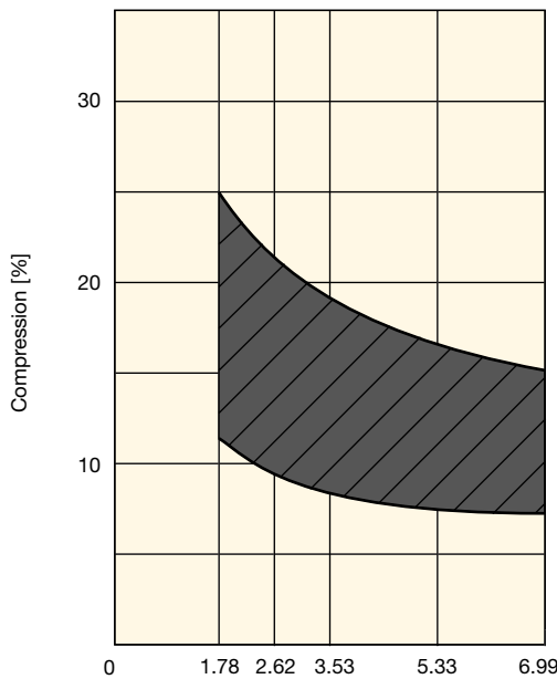
O-Ring cross-section d_2 [mm]
