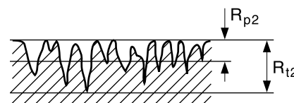
Surfaces produced by normal machining
