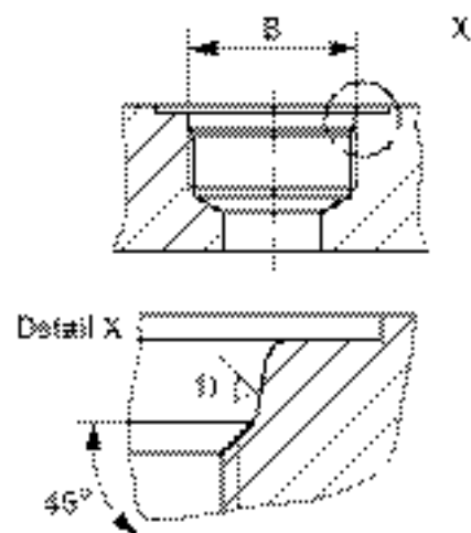
Fig. 4.1 Threaded connector with conical counterbore
