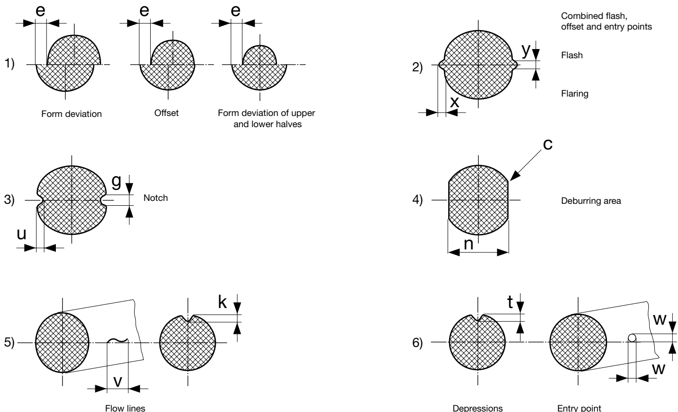
Fig. 9.1 Form and surface finish defects
