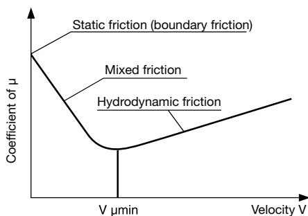
Fig. 8.18 Stribeck curve
