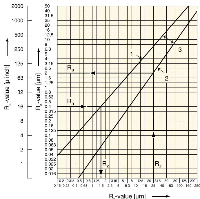
Surfaces produced by normal machining
